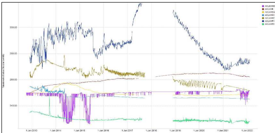
Figure 6: Cockatoo Creek Spring Complex EWS Groundwater Pressure Data
