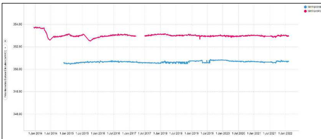
Figure 3: Abyss and Lucky Last EWS Groundwater Pressure Data at MHTGWP01 and MHTGWH01
