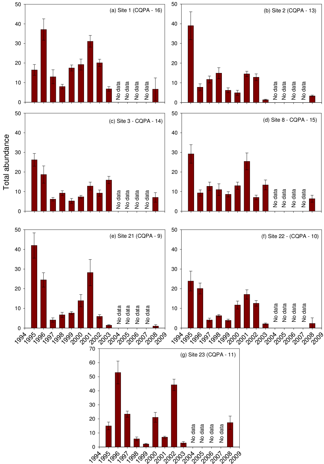
Figure 9. Mean ( \pm SE) macroinvertebrate abundance at different sites from 1995-2003 & 2008. No data available from 2004-07. Data collected from other sources (Alquezar and Small 2006) ( n = 10 , 94-03; n = 3 , 2003).
